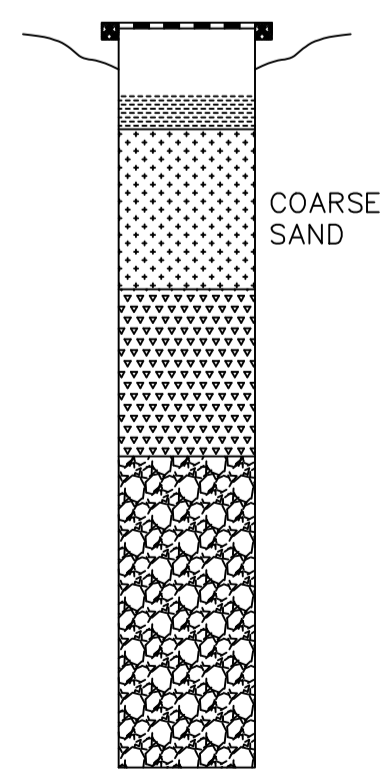
C.S RAINWATER HARVESTING
